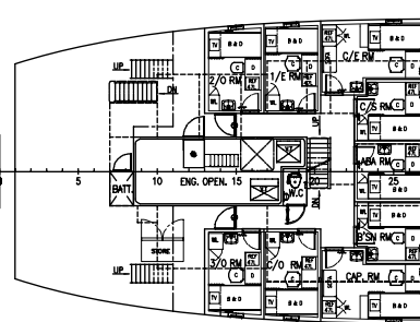
BOAT DECK
