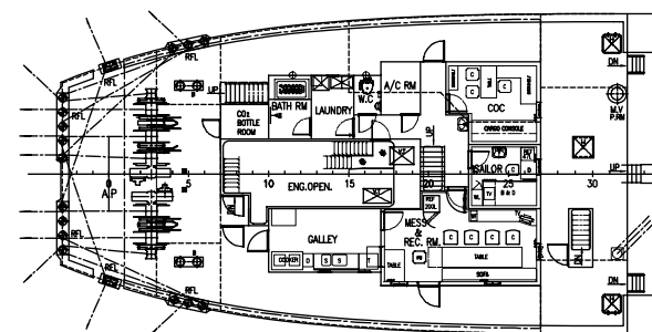
POOP DECK
