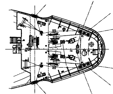
UPPER DECK
