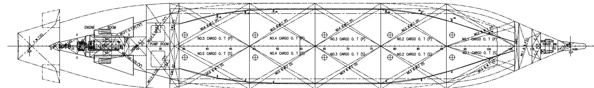
HOLD PLAN
